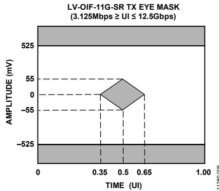
Figure 42. Receiver Eye Mask
