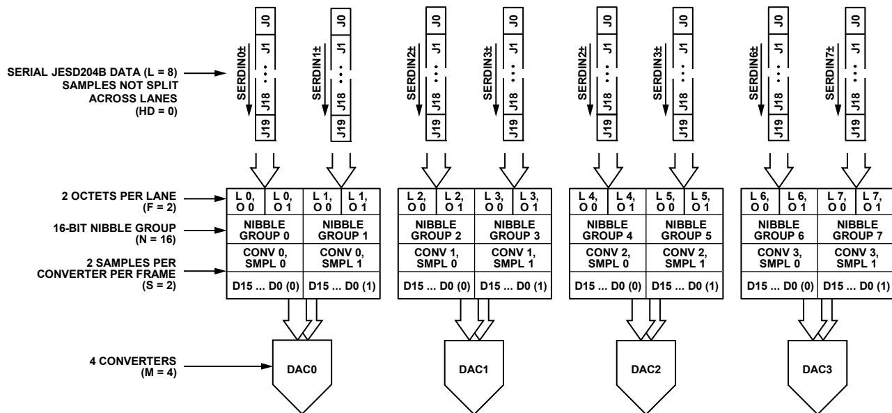
Figure 59. JESD204B Mode 1 Data Deframing
