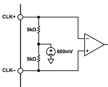
Figure 74. Clock Receiver Input Simplified Equivalent Circuit
