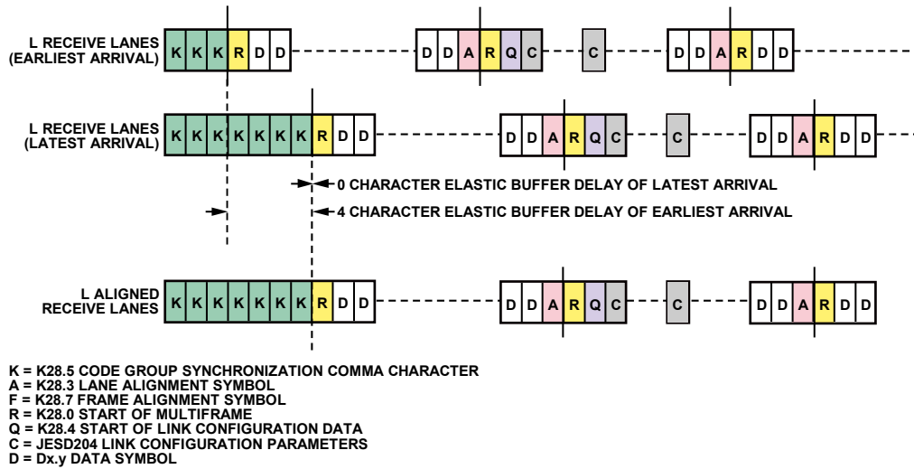
Figure 48. Lane Alignment During ILAS
