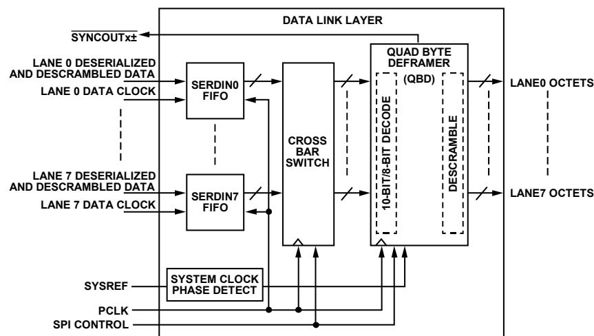
Figure 47. Data Link Layer Block Diagram
