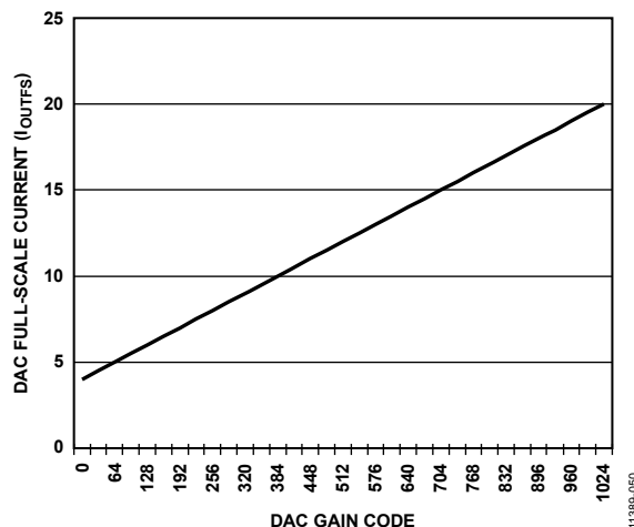
Figure 79. DAC Full-Scale Current ( I_{OUTFS} ) vs. DAC Gain Code
