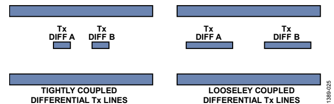
Figure 86. Tightly Coupled vs. Loosely Coupled Differential Traces
