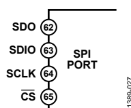
Figure 35. SPI Pins
