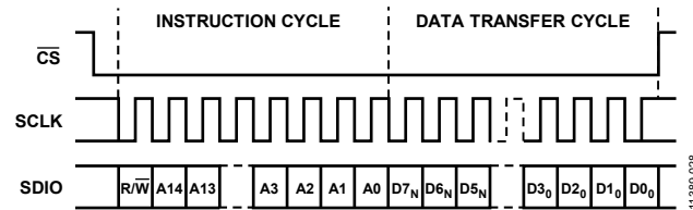
Figure 36. Serial Register Interface Timing, MSB First, Address Increment Bits = 0
