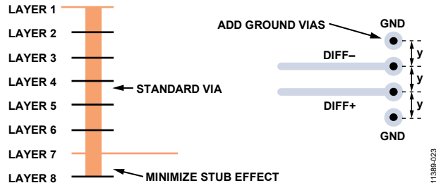
Figure 84. Minimizing Stub Effect and Adding Ground Vias for Differential Stripline Traces
