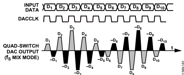
Figure 81. Mix Mode Waveform
