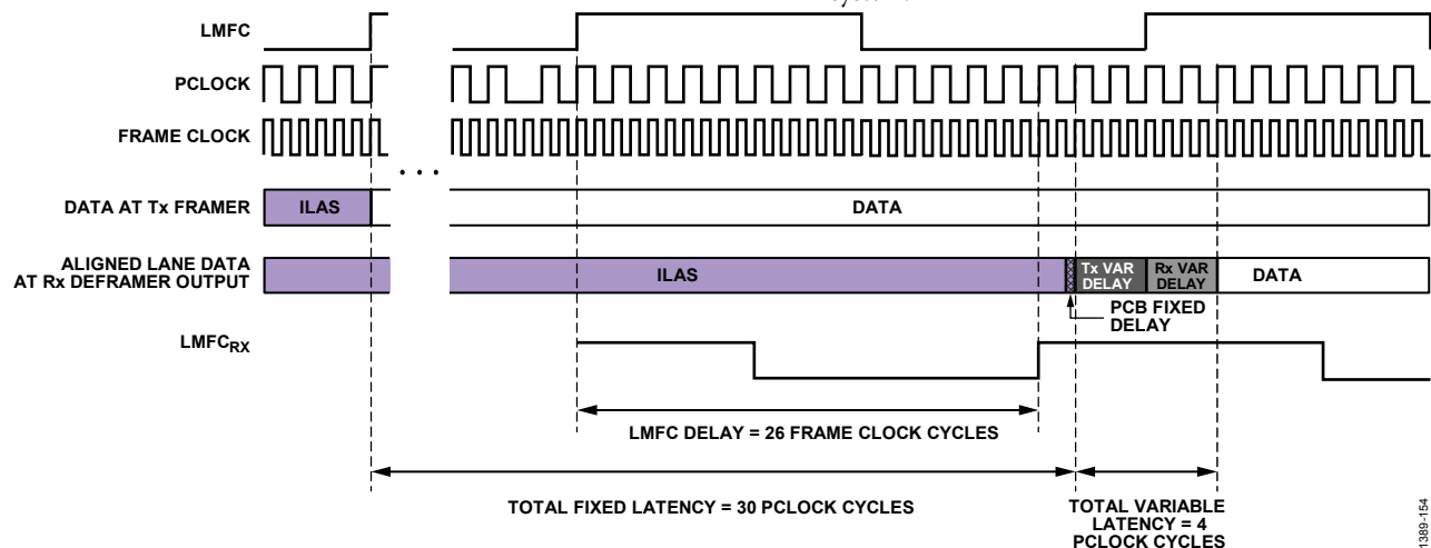
Figure 53. LMFC_DELAY Calculation Example
