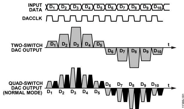
Figure 80. Two-Switch and Quad-Switch DAC Waveforms
