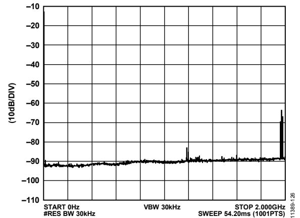
Figure 26. Single Tone SFDR f_{DAC} = 1966.08\text{ MHz} , 4x Interpolation, f_{OUT} = 10\text{ MHz} , -14 dBFS
