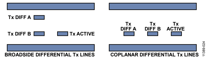
Figure 85. Broadside vs. Coplanar Differential Stripline Routing Techniques
