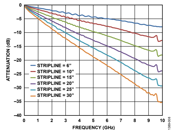
Figure 44. Insertion Loss of 50 \Omega Striplines on FR-4
