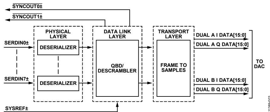
Figure 40. Functional Block Diagram of Serial Link Receiver
