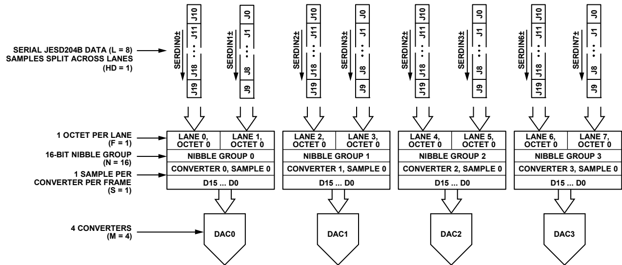
Figure 58. JESD204B Mode 0 Data Deframing
