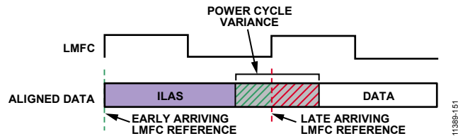
Figure 50. Link Delay > LMFC Period Example
