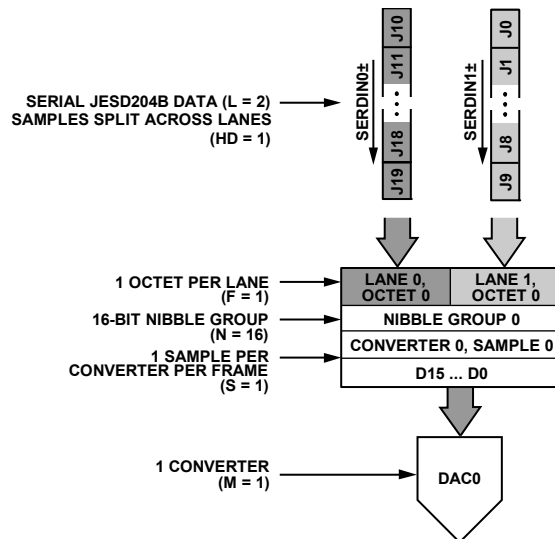
Figure 65. JESD204B Mode 9 Data Deframing
