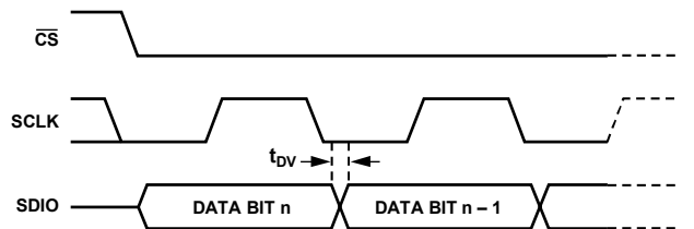
Figure 38. Timing Diagram for Serial Port Register Read
