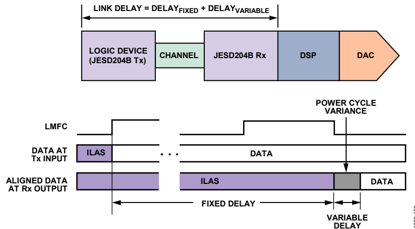
Figure 52. JESD204B Link Delay = Fixed Delay + Variable Delay
