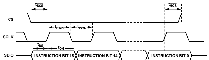
Figure 39. Timing Diagram for Serial Port Register Write
