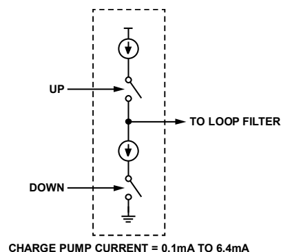
Figure 76. Charge Pump
