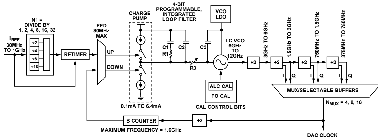
Figure 77. Device Clock PLL Block Diagram
