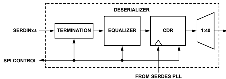
Figure 41. Deserializer Block Diagram
