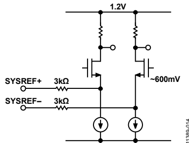
Figure 49. \text{SYSREF}\pm Input Circuit
