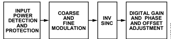
Figure 67. Block Diagram of the Digital Datapath
