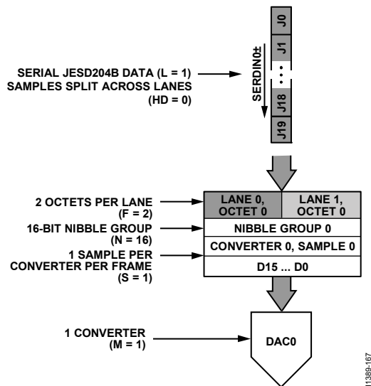
Figure 66. JESD204B Mode 10 Data Deframing
