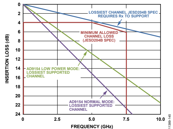
Figure 43. Insertion Loss Allowed
