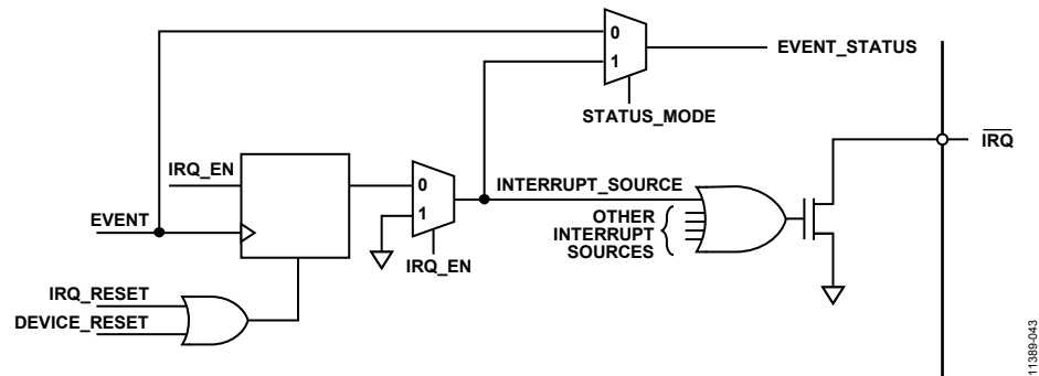
Figure 73. Simplified Schematic of \overline{\text{IRQ}} Circuitry
