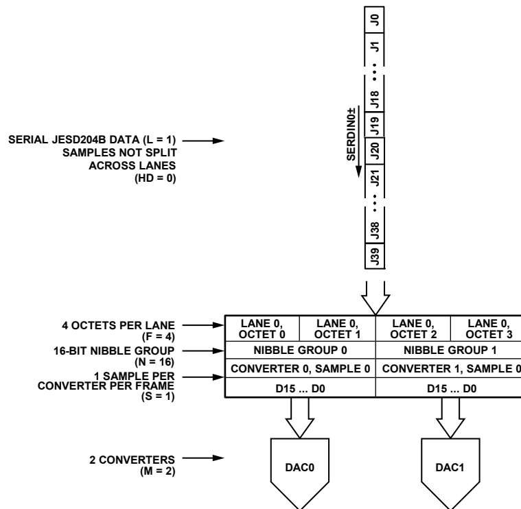
Figure 64. JESD204B Mode 7 Data Deframing
