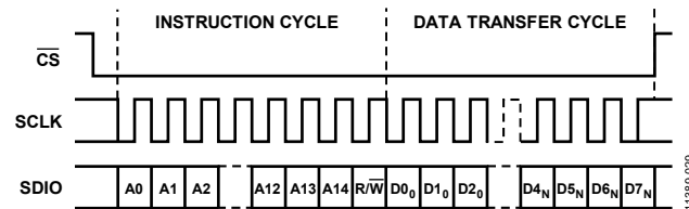
Figure 37. Serial Register Interface Timing, LSB First, Address Increment Bits = 1
