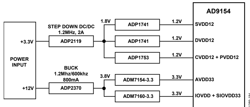
Figure 83. Power Supply Connections
