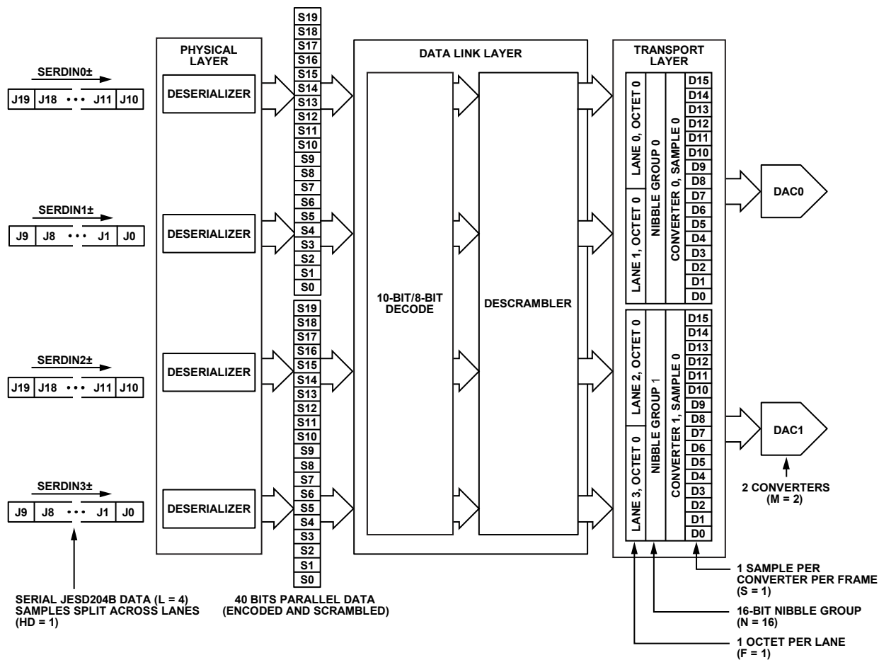
Figure 57. JESD204B Mode 4 Data Deframing
