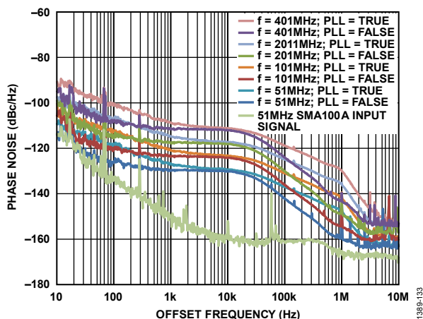
Figure 33. Single Tone Phase Noise vs. Offset Frequency at 4 Different f_{OUT} Rates, f_{DAC} = 1.96608 \text{ GHz} , PLL On and Off
