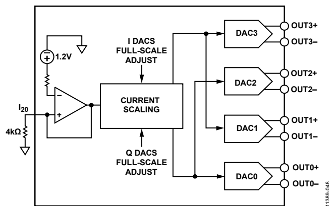
Figure 78. Simplified Block Diagram of the DAC Core
