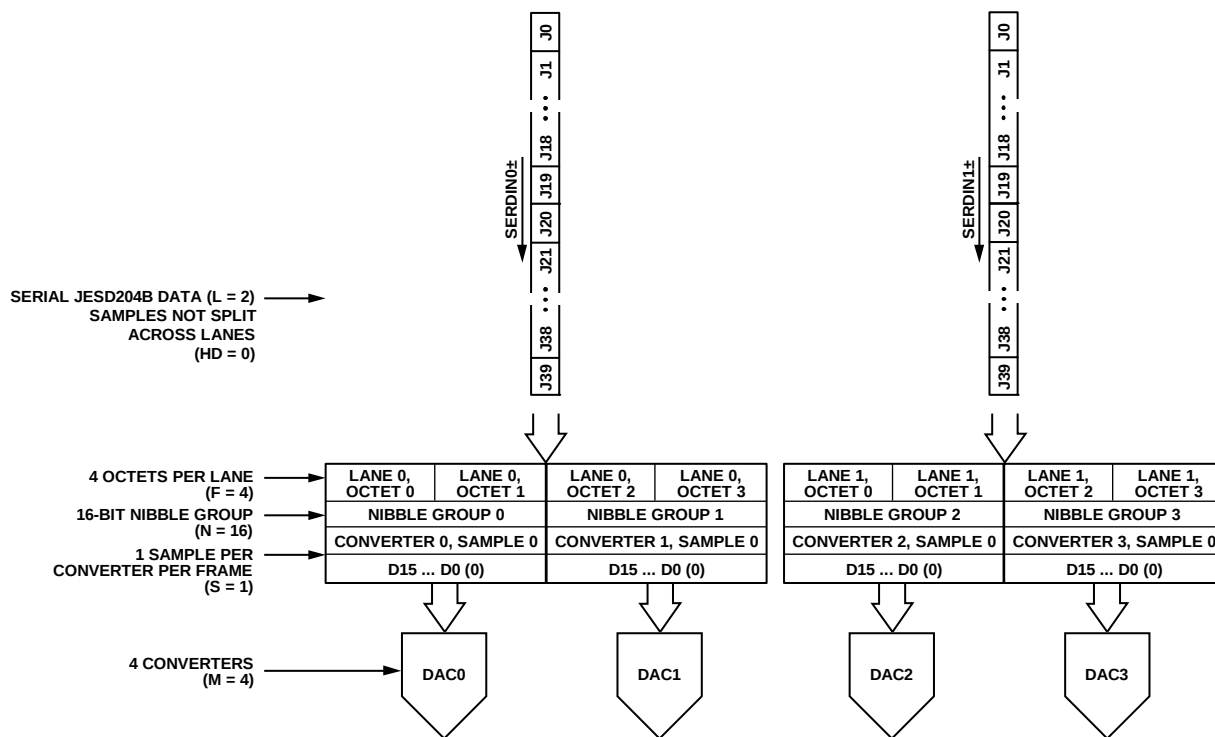
Figure 61. JESD204B Mode 3 Data Deframing
