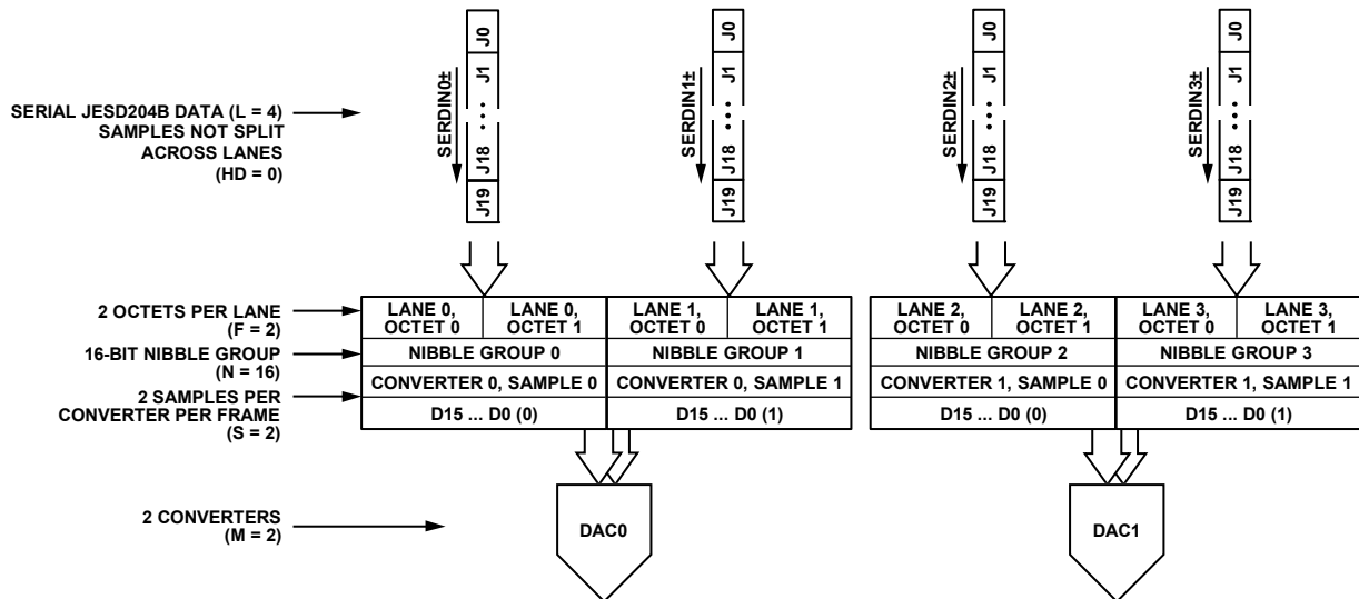
Figure 62. JESD204B Mode 5 Data Deframing
