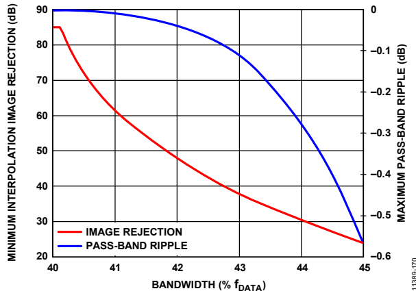
Figure 69. Interpolation Filter Performance Beyond Specified Bandwidth
