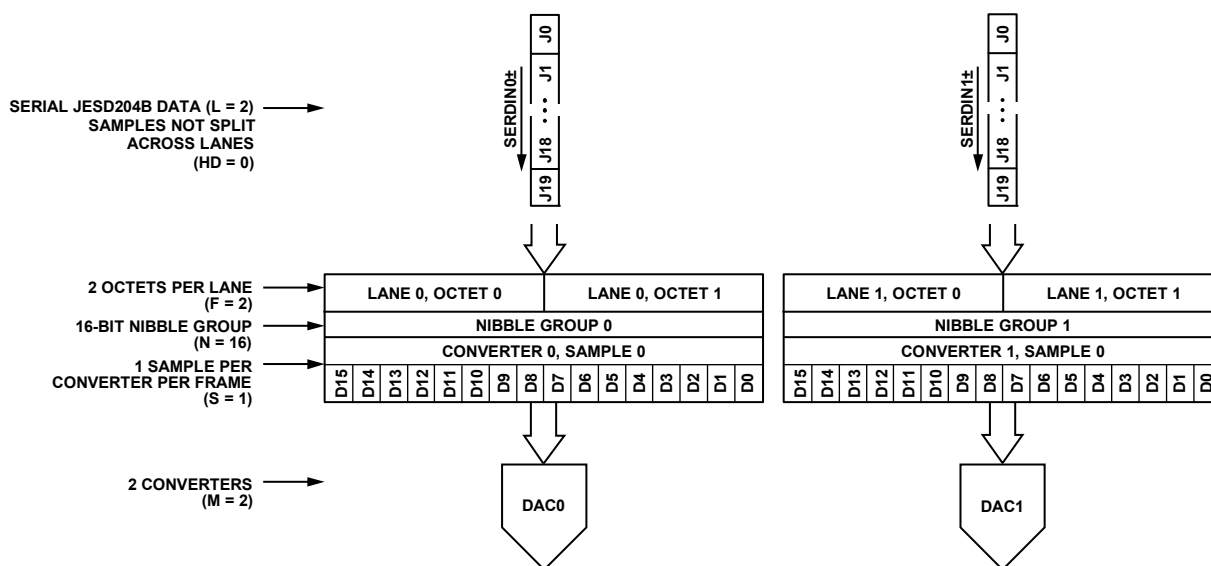
Figure 63. JESD204B Mode 6 Data Deframing
