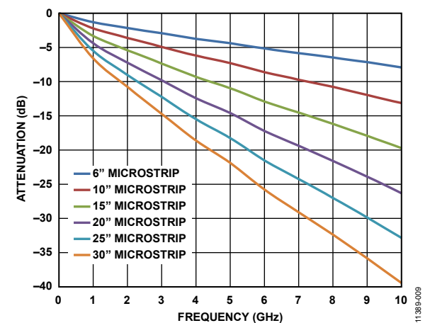
Figure 45. Insertion Loss of 50 \Omega Microstrips on FR-4
