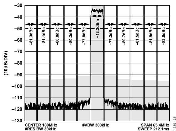
Figure 34. 1C 256 Point Quadrature Amplitude Modulation (QAM) Signal ACLR Performance, f_{IF} = 180 \text{ MHz} , f_{DAC} = 1966.08 \text{ MHz}
