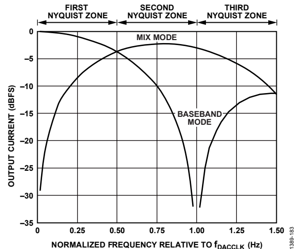
Figure 82. Sinc Roll-Off for Normal Mode and Mix-Mode Operation
