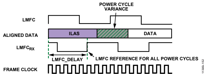
Figure 51. LMFC DELAY to Compensate for Link Delay > LMFC
