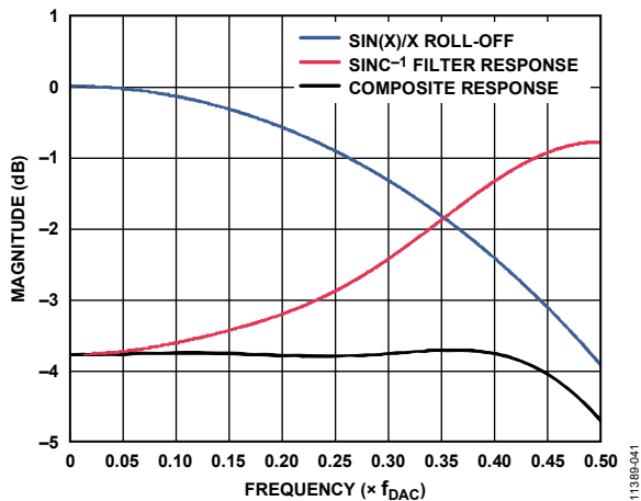
Figure 71. Responses of \sin(x)/x Roll-Off, the \text{Sinc}^{-1} Filter, and the Composite of the Two Input Signal Power Detection and Protection
