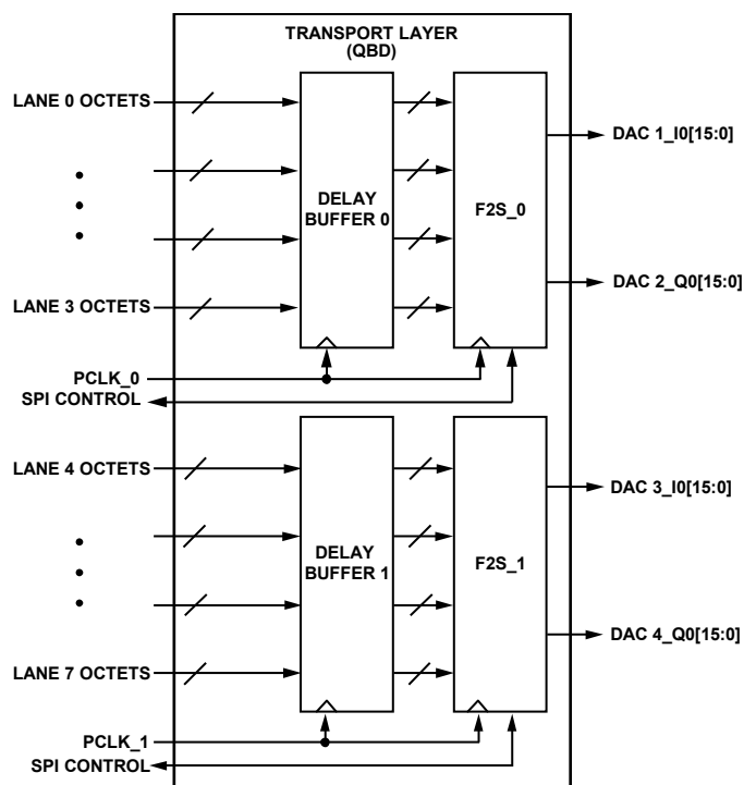
Figure 56. Transport Layer Block Diagram
