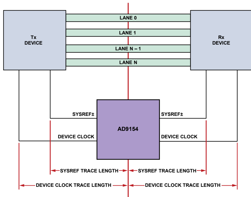
Figure 87. SYSREF± Signal and Device Clock Trace Length
