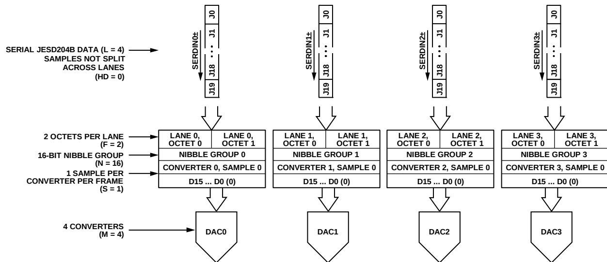
Figure 60. JESD204B Mode 2 Data Deframing
