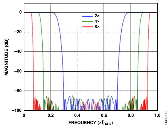
Figure 68. All Band Responses of Interpolation Filters
