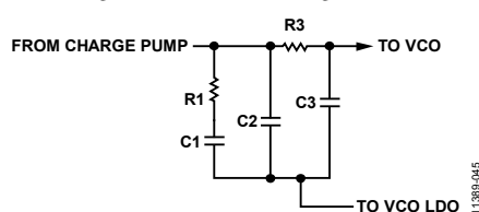
Figure 75. Loop Filter
