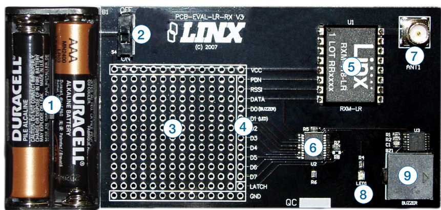
Figure 4: LR Receiver Evaluation Board
