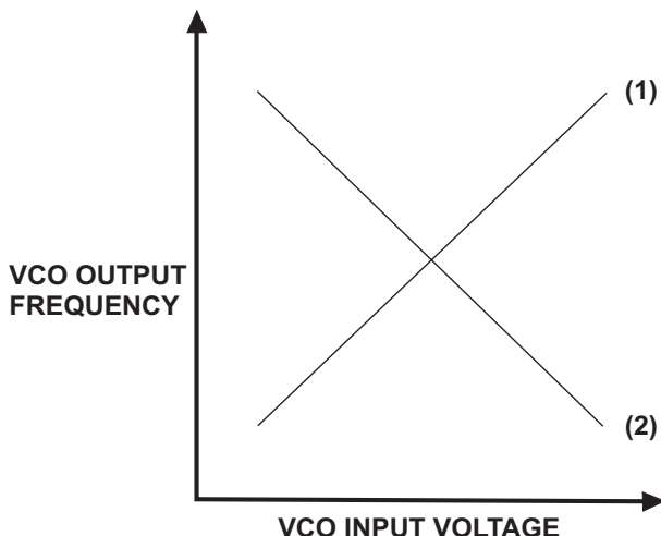
Figure 10: VCO Characteristics
