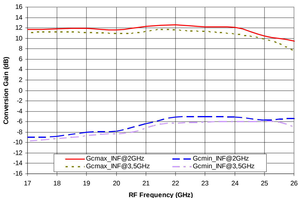
Figure 2: Conversion Gain in Infradyne Mode versus Frequency F_{RF} = 2 \times F_{LO} - F_{IF} , F_{IF} = 2.0 \text{ \& } 3.5\text{GHz} , GC2 = GC3 = -1.5 \text{ \& } 0.5\text{V}
