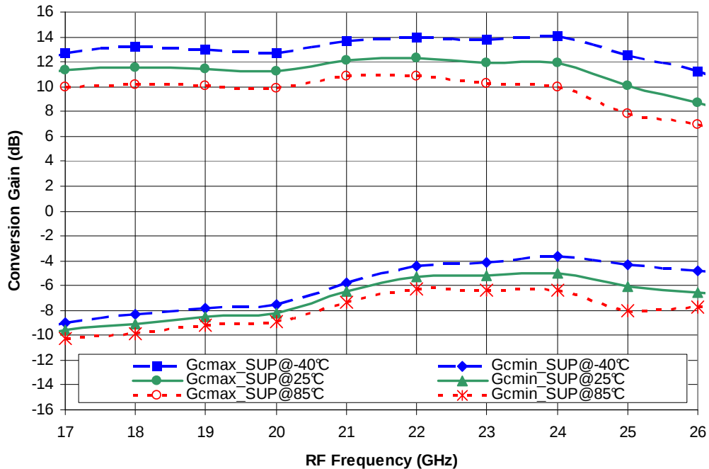
Figure 9: Conversion Gain in Supradyn Mode versus Temperature & Frequency F_{RF} = 2 \times F_{LO} + F_{IF} , F_{IF} = 2.0\text{GHz} , GC2 = GC3 = -1.5 \text{ \& } 0.5\text{V}
