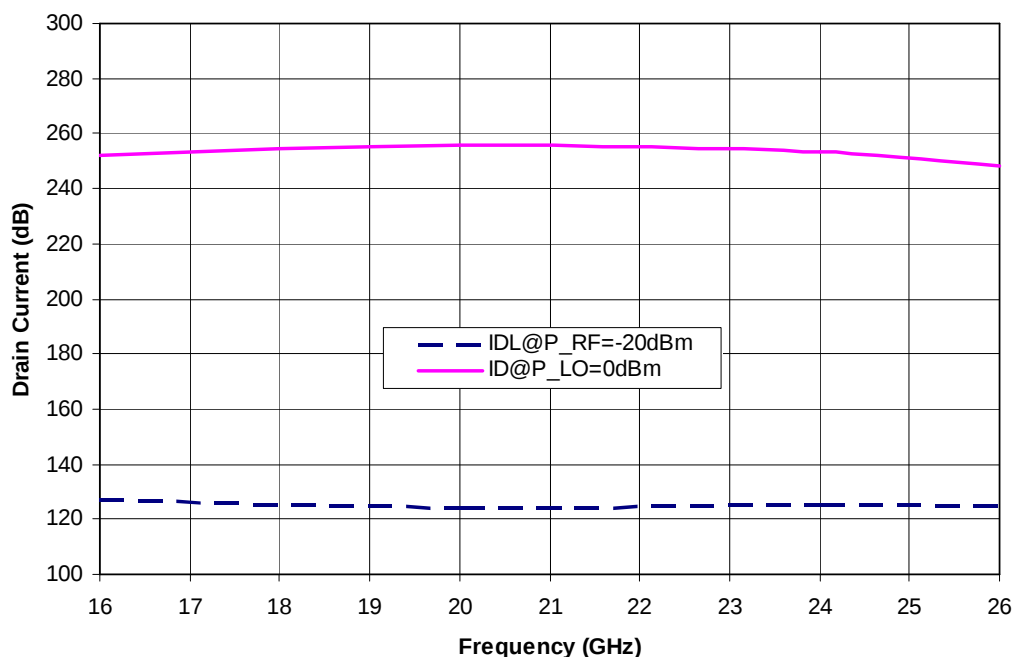
Figure 4: Drain Currents versus Frequency
