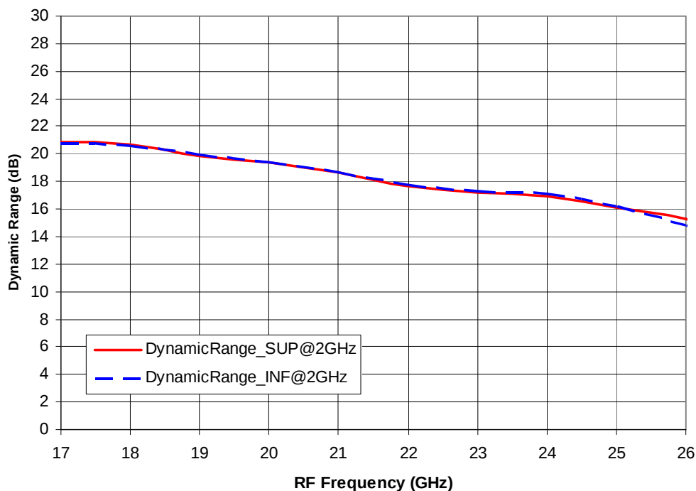
Figure 3: Dynamic Range (Gcmax – Gcmin) versus Frequency
