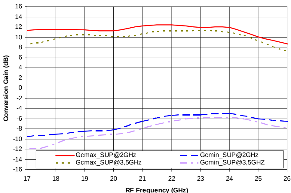
Figure 1: Conversion Gain in Supradyn Mode versus Frequency F_{RF} = 2 \times F_{LO} + F_{IF} , F_{IF} = 2.0 \text{ \& } 3.5\text{GHz} , GC2 = GC3 = -1.5 \text{ \& } 0.5\text{V}
