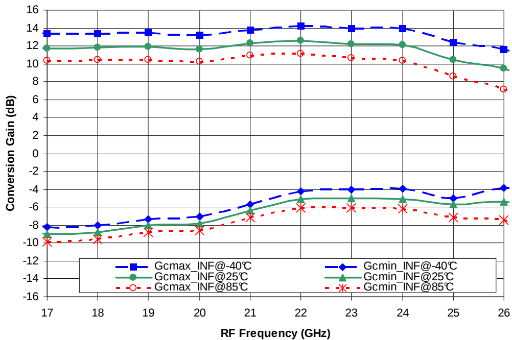
Figure 10: Conversion Gain in Infradyne Mode versus Temperature & Frequency F_{RF} = 2 \times F_{LO} - F_{IF} , F_{IF} = 2.0\text{GHz} , GC2 = GC3 = -1.5 \text{ \& } 0.5\text{V}
