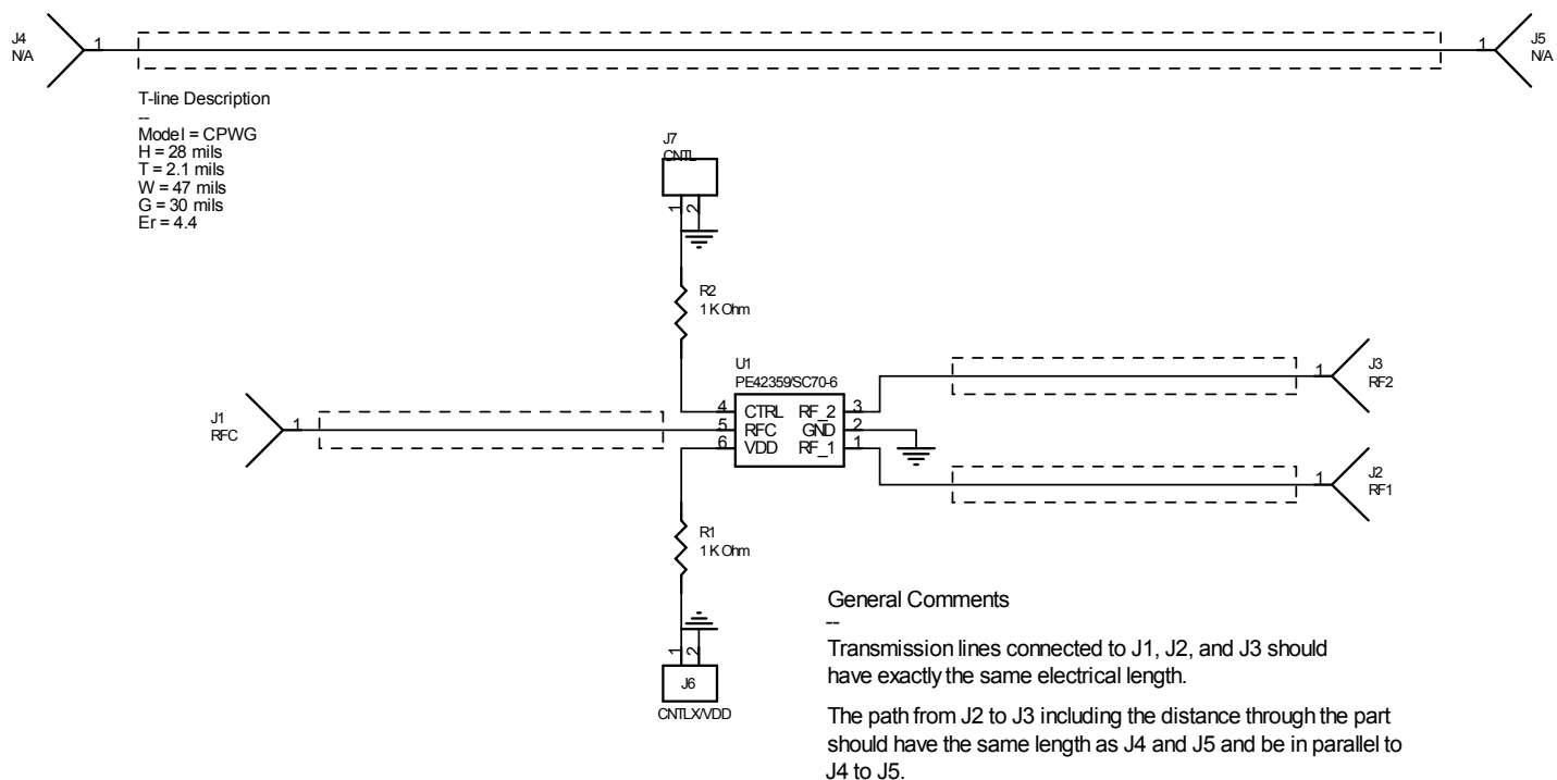
Figure 27. Evaluation Board Schematic
