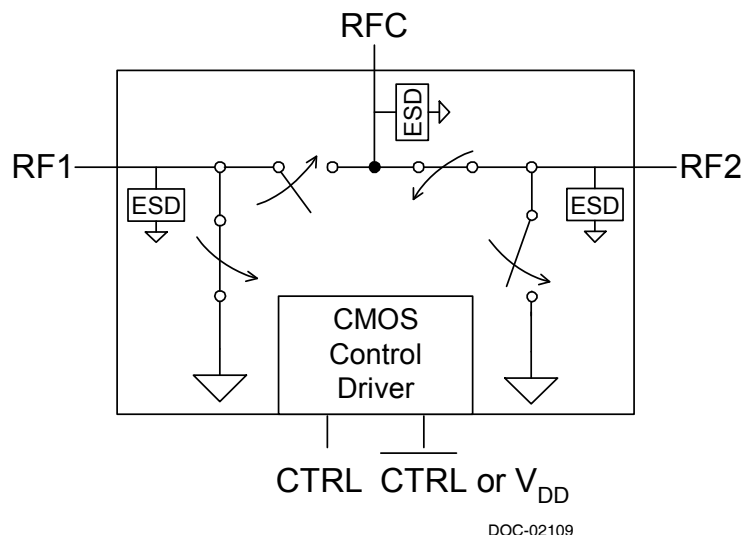
Figure 1. Functional Diagram
