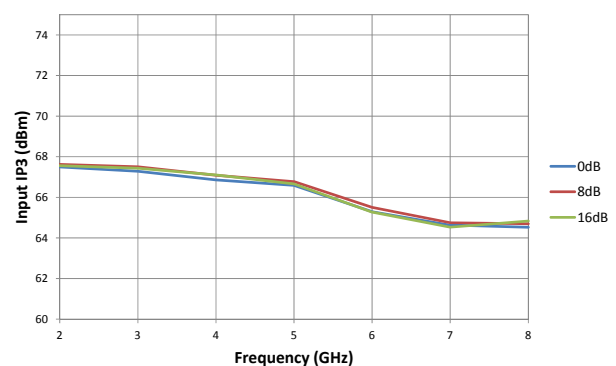
Figure 29. IIP3 vs. Attenuation Setting
