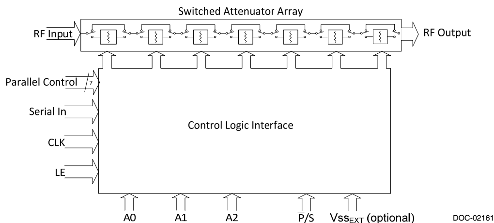
Figure 2. Functional Diagram
