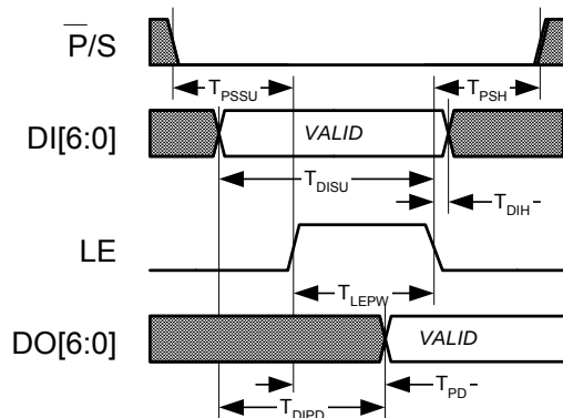
Figure 6. Latched-Parallel/Direct-Parallel Timing Diagram
