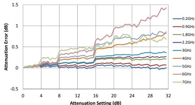
Figure 14. 0.5 dB Attenuation Error vs. Frequency
