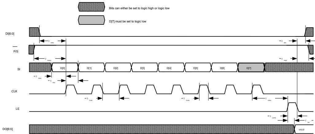
Figure 5. Serial Timing Diagram
