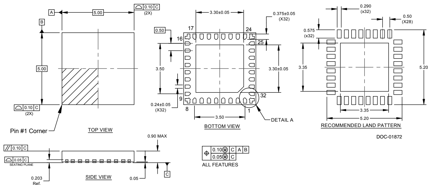
Figure 33. Package Drawing 32-lead 5x5 QFN
