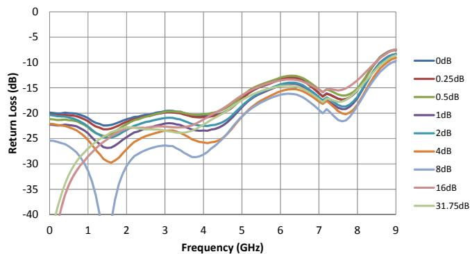
Figure 20. Input Return Loss vs. Attenuation Setting
