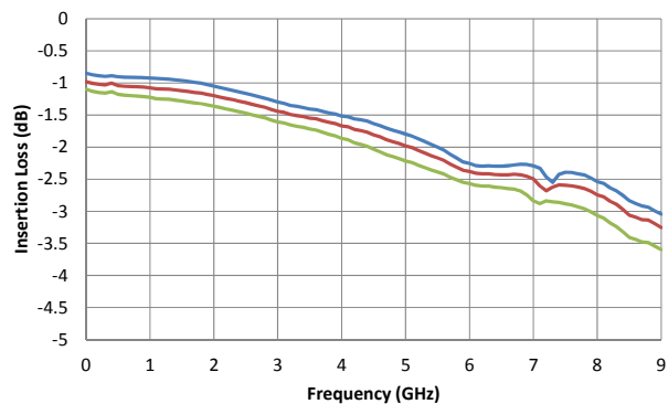
Figure 19. Insertion Loss vs. Temperature
