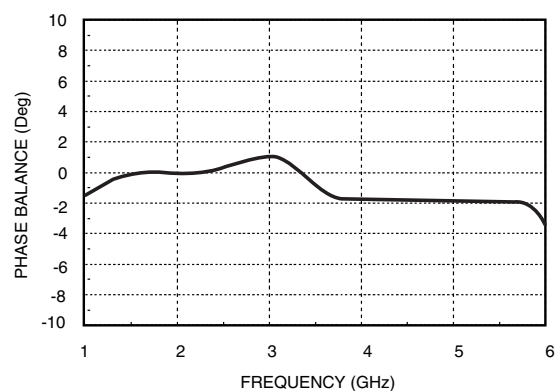
Phase Balance
