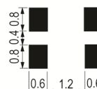
Underside View
