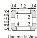
Underside View
