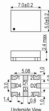
Underside View
