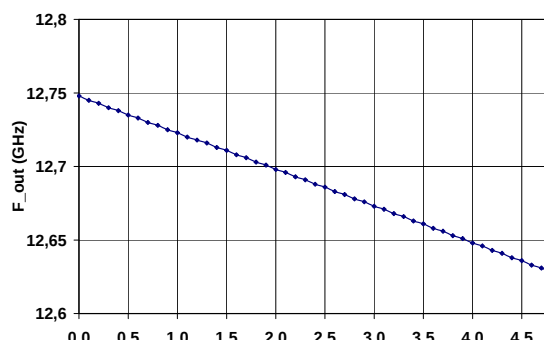
Typical free running VCO F out (V mt ) tuning
