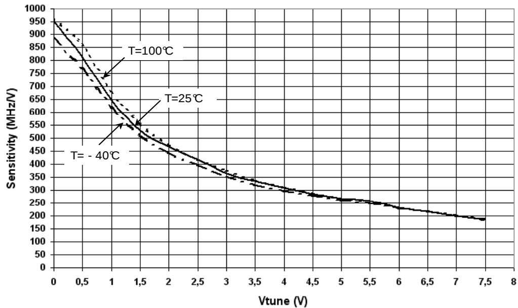
Sensitivity versus Vtune
