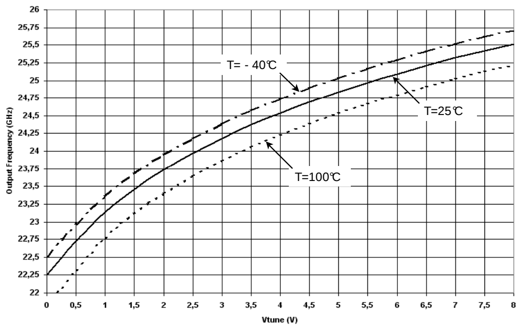
Output Frequency versus Vtune
