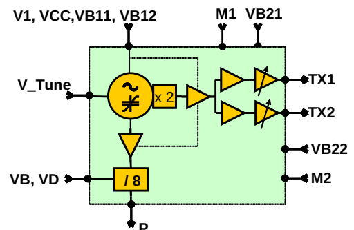
Block Diagram
