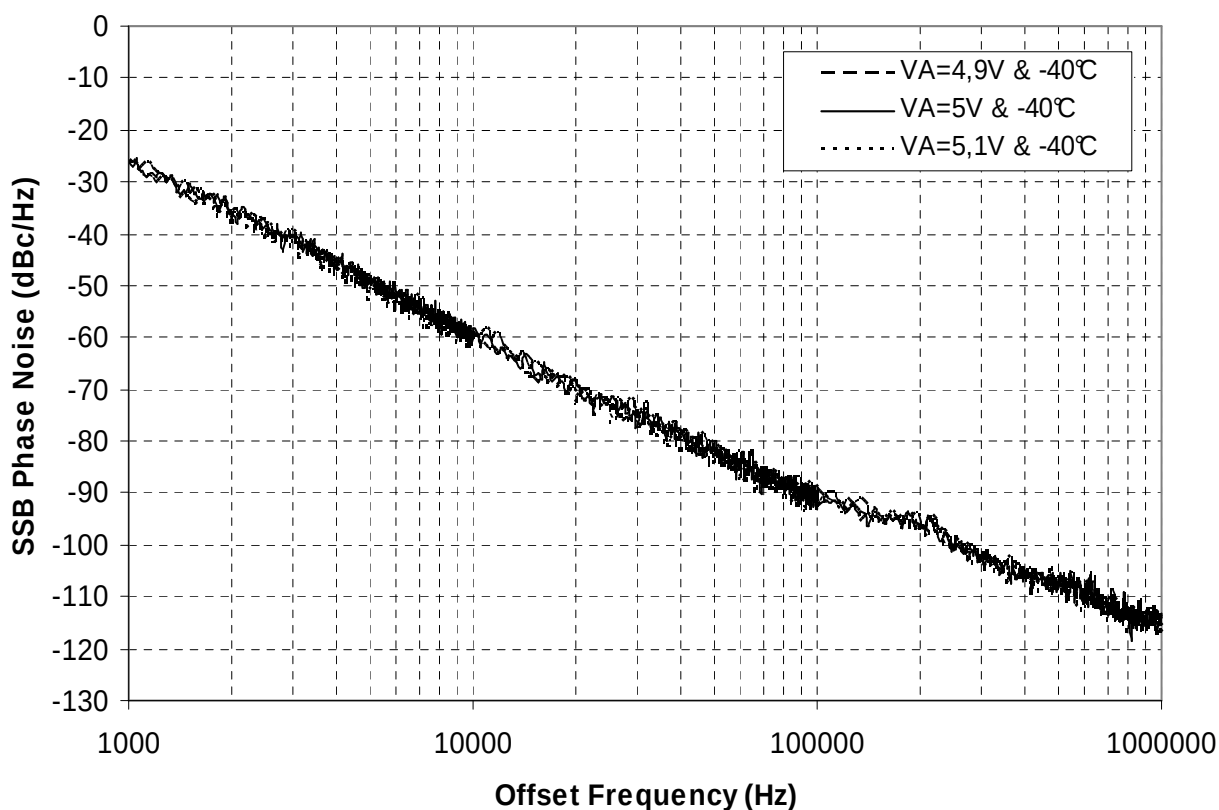
Phase Noise versus Offset frequency from carrier &amp; +V @ Vt = 3V, Top = -40°C
