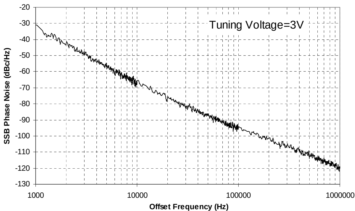
Phase Noise versus Offset frequency from carrier &amp; +V @ Vt = 3V, Top = -40°C
