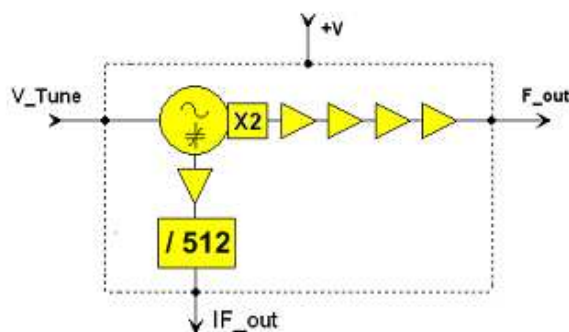
Multifunction block diagram
