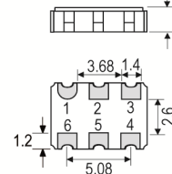
Underside View
