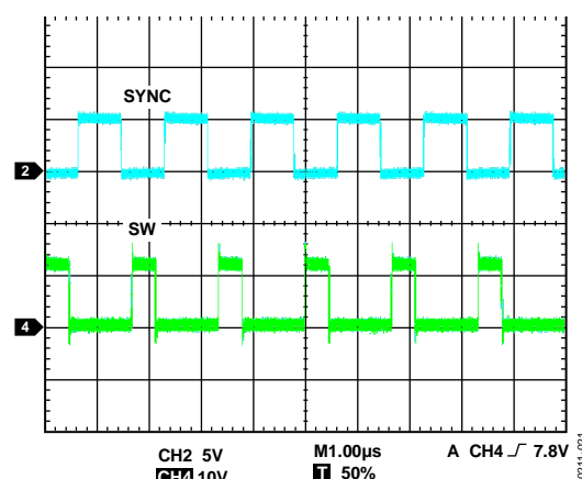
Figure 21. External Synchronization
