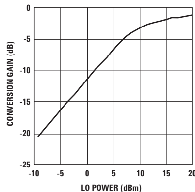
Figure 20. Conversion Gain vs. LO power. RF = 21\text{ GHz} ( -20\text{ dBm} ), LO = 20\text{ GHz} .
