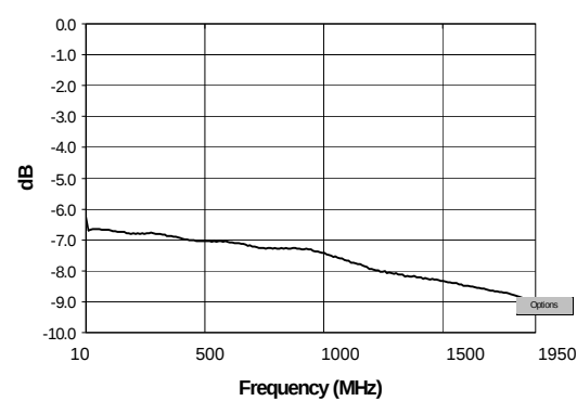
Conversion Loss
