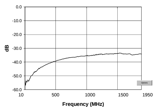
L-X Isolation
