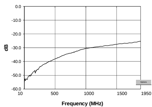
L-R Isolation
