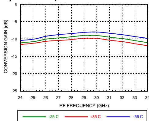
Conversion Gain vs. Temperature Upconverter, LO= 9 GHz
