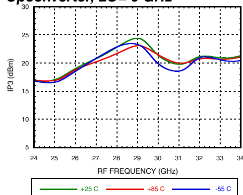
Input IP3 vs. Temperature Upconverter, LO= 9 GHz
