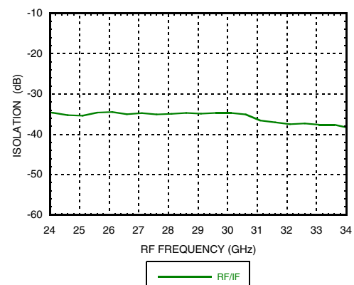
Isolation RF/IF
