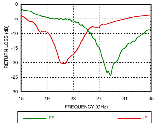
RF and IF Return Loss
