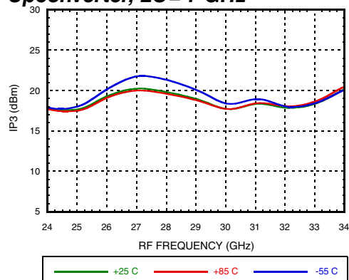
Input IP3 vs. Temperature Upconverter, LO= 7 GHz
