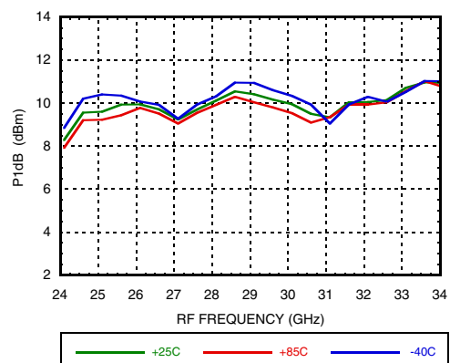
Input P1dB vs. Temperature @ LO= 9 GHz
