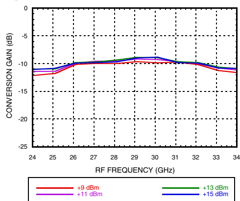
Conversion Gain vs. LO Power Upconverter, LO= 9 GHz
