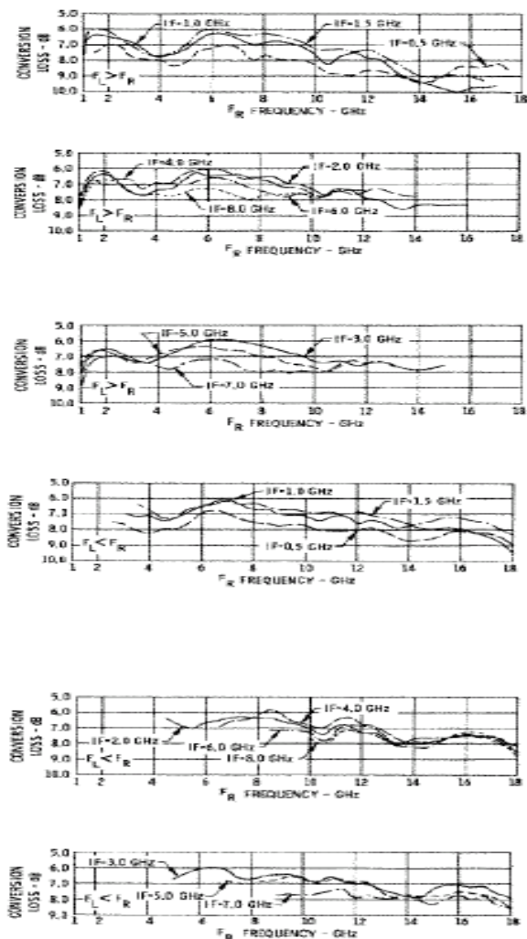
Conversion Loss vs. Frequency, LO @ +13 dBm
