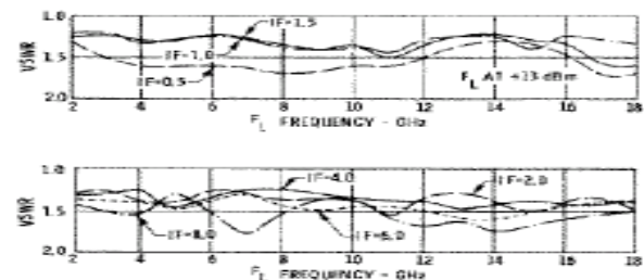
I-Port VSWR vs. Frequency LO @ +13 dBm
