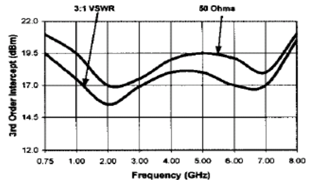
3rd Order Intercept vs. IF Port Termination 3
