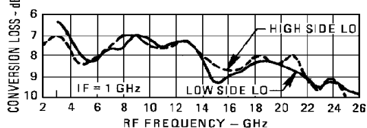
Conversion Loss vs. Frequency
