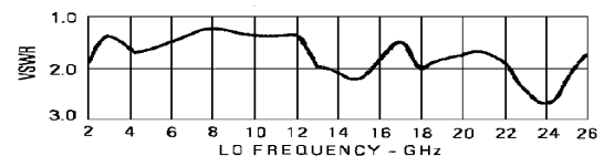
L-Port VSWR
