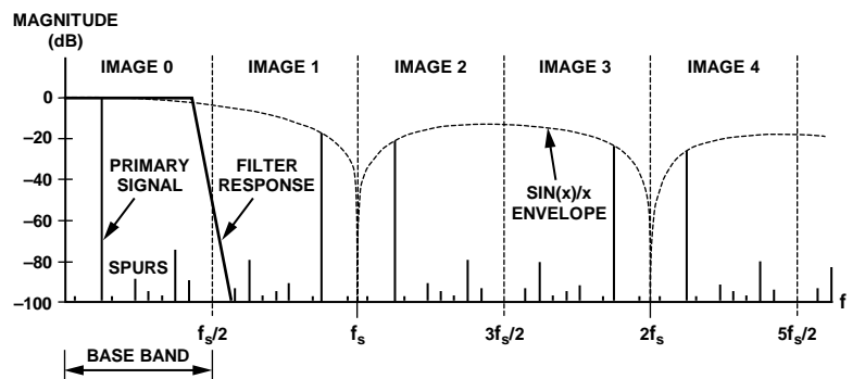
Figure 31. DAC Spectrum vs. Reconstruction Filter Response
