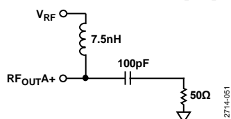
Figure 53. Optimum Output Stage
