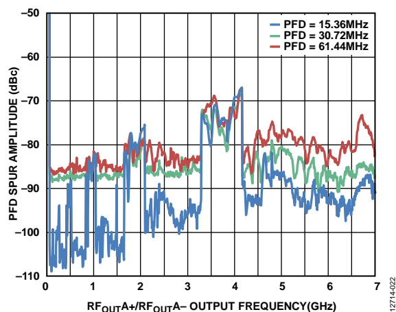
Figure 23. PFD Spur Amplitude vs. RF_{OUTA+}/RF_{OUTA-} Output Frequency; PFD = 61.44 MHz, PFD = 30.72 MHz, and PFD = 15.36 MHz; Loop Filter = 20 kHz
