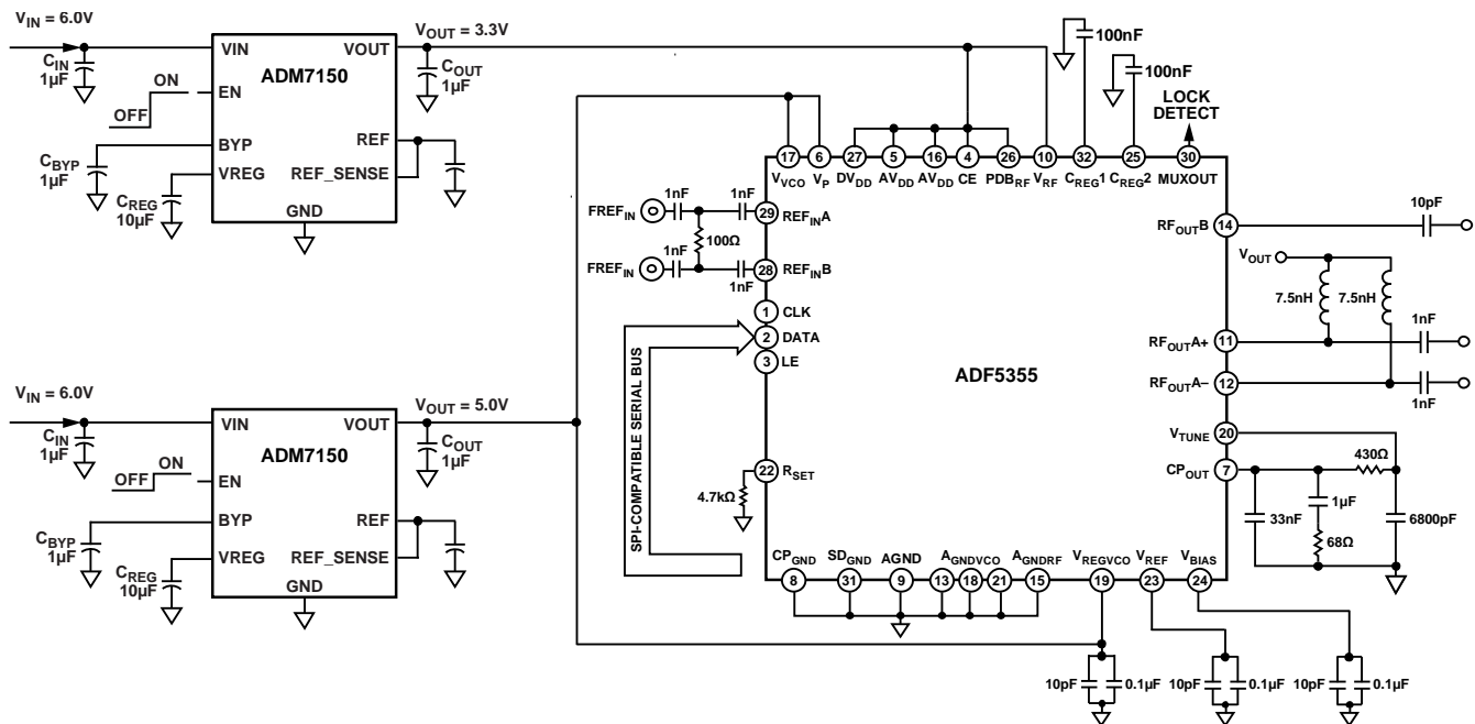
Figure 52. ADF5355 Power Supplies
