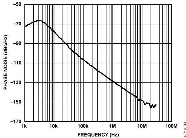
Figure 14. Closed-Loop Phase Noise, RF_{OUTB} = 10 GHz, 2 \times VCO , VCO = 5.0 GHz, PFD = 61.44 MHz, Loop Bandwidth = 2 kHz
