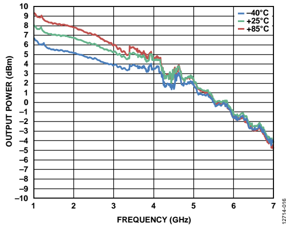
Figure 16. Output Power vs. Frequency, RF_{OUTA+}/RF_{OUTA-} (7.5 nH Inductors, 10 pF Bypass Capacitors, Board Losses De-Embedded)
