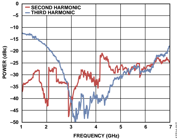
Figure 17. RF_{OUTA+}/RF_{OUTA-} Harmonics vs. Frequency (7.5 nH Inductors, 10 pF Bypass Capacitors, Board Losses De-Embedded)
