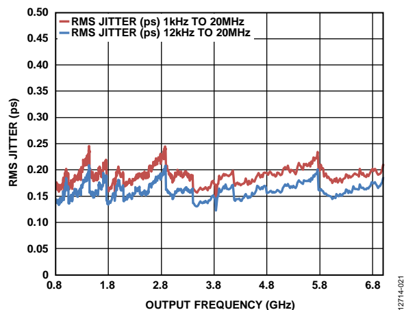
Figure 22. RMS Jitter vs. Output Frequency, PFD Frequency = 61.44 MHz, Loop Filter = 20 kHz
