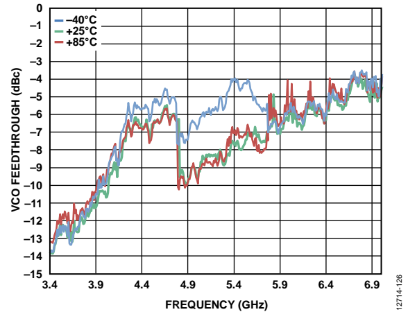
Figure 20. VCO Feedthrough at RF_{OUTB} (De-Embedded) vs. Fundamental VCO Frequency
