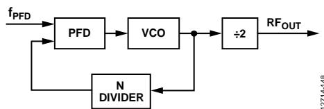
Figure 51. Loop Closed Before Output Divider
