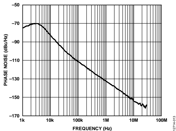
Figure 13. Closed-Loop Phase Noise, RF_{OUTB} = 6.8 GHz, 2 \times VCO , VCO = 3.4 GHz, PFD = 61.44 MHz, Loop Bandwidth = 2 kHz
