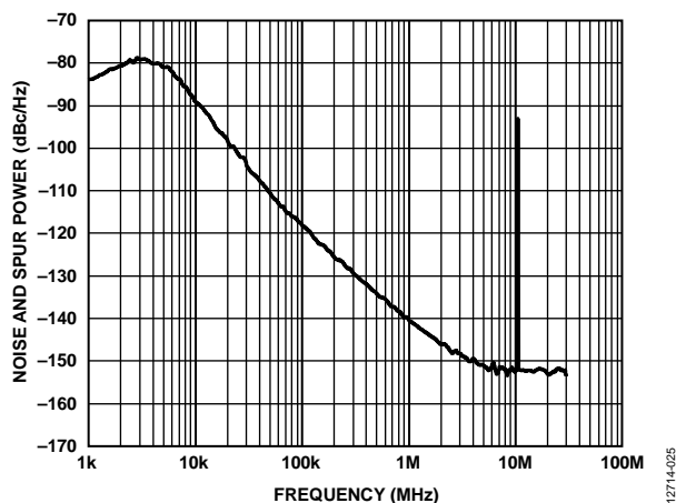
Figure 26. Fractional-N Spur Performance, RF_{OUTA+} = 2.591 GHz, REF_{IN} = 122.88 MHz, PFD = 61.44 MHz, Output Divide by 2 Selected, Loop Filter Bandwidth = 2 kHz, Channel Spacing = 20 kHz
