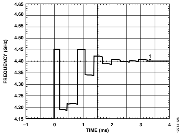
Figure 28. Lock Time for 100 MHz Jump from 3500 MHz to 7000 MHz, Loop Bandwidth = 20 kHz
