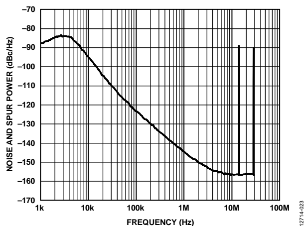
Figure 24. Fractional-N Spur Performance, GSM1800 Band, RF_{OUTA+} = 1550.2 MHz, REF_{IN} = 122.88 MHz, PFD = 61.44 MHz, Output Divide by 4 Selected, Loop Filter Bandwidth = 2 kHz, Channel Spacing = 20 kHz
