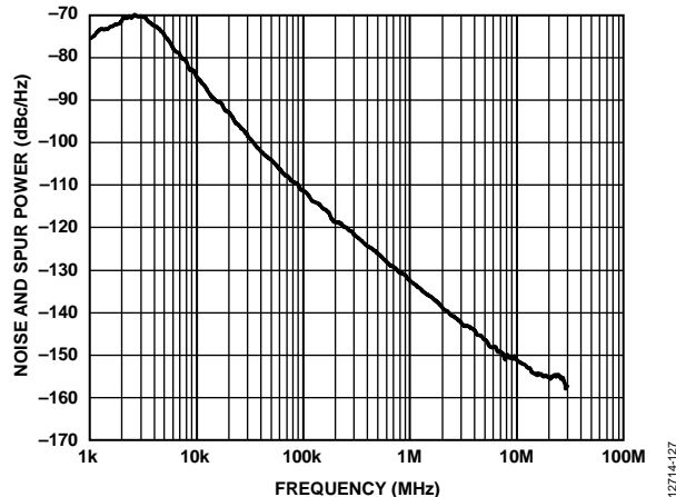
Figure 27. Fractional-N Spur Performance, RF_{OUTA+} = 5.8 GHz, REF_{IN} = 122.88 MHz, PFD = 61.44 MHz, Output Divide by 2 Selected, Loop Filter Bandwidth = 2 kHz, Channel Spacing = 20 kHz
