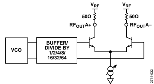
Figure 34. Output Stage
