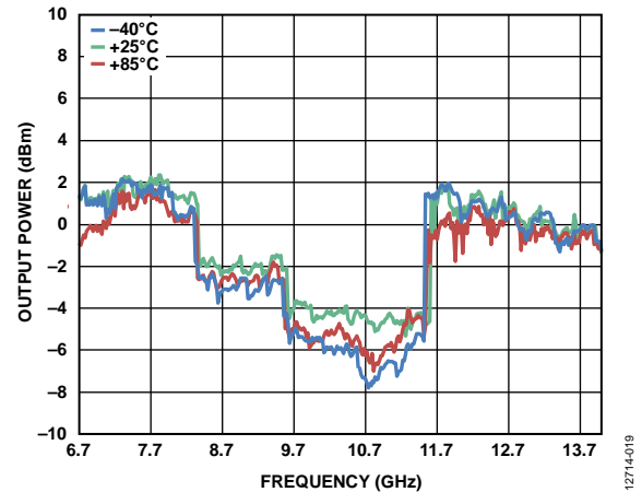
Figure 19. Output Power vs. Frequency, RF_{OUTB} (10 pF Bypass Capacitor, De-Embedded)
