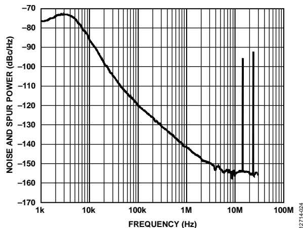
Figure 25. Fractional-N Spur Performance, W-CDMA Band, RF_{OUTA+} = 2113.5 MHz, REF_{IN} = 122.88 MHz, PFD = 61.44 MHz, Output Divide by 2 Selected, Loop Filter Bandwidth = 2 kHz, Channel Spacing = 20 kHz
