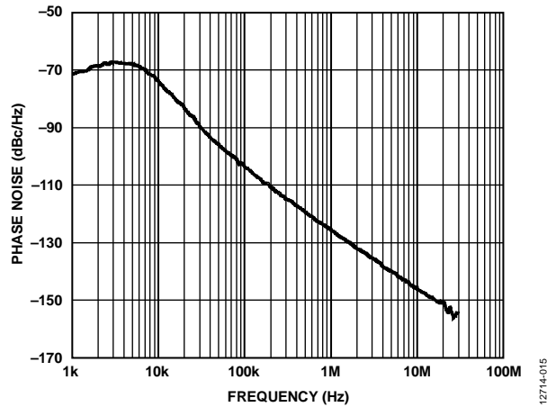
Figure 15. Closed-Loop Phase Noise, RF_{OUTB} = 13.6 GHz, 2 \times VCO , VCO = 6.8 GHz, PFD = 61.44 MHz, Loop Bandwidth = 2 kHz
