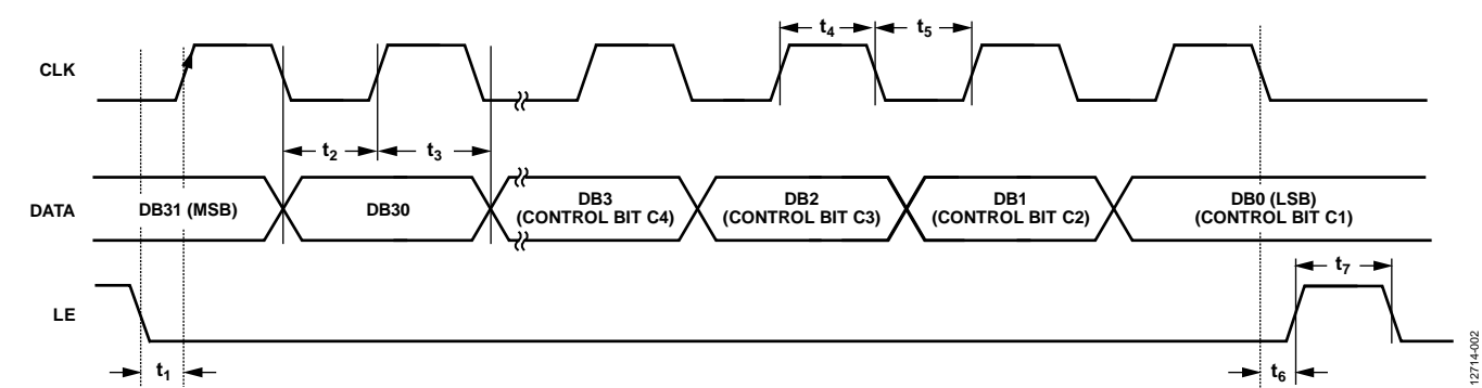
Figure 2. Timing Diagram
