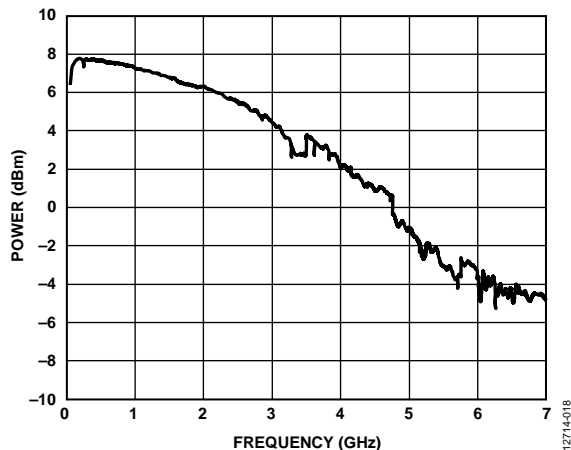
Figure 18. RF_{OUTA+}/RF_{OUTA-} Power vs. Frequency (100 nH Inductors, 100 pF Bypass Capacitors, Board Measurement)
