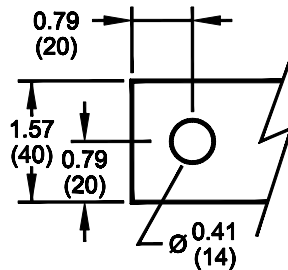
800/1000A BUS BAR: 8x40
