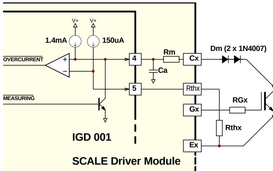
Fig. 4 Collector-sense circuit principle
