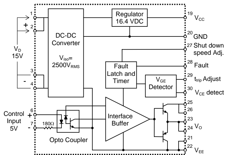
Figure 1: VLA500-01/VLA502-01 Block Diagram
