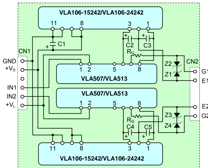
Figure 3: BG2C Schematic and Component Selection
