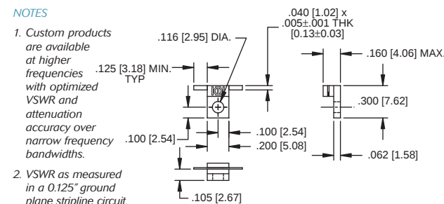
PPA10 OUTLINE
