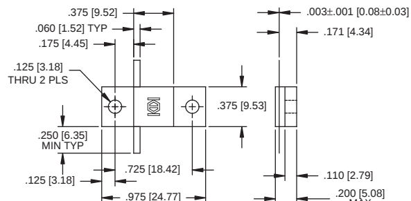
PPA50 OUTLINE
