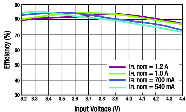
Figure 4. Flash Mode Efficiency vs Input Voltage
