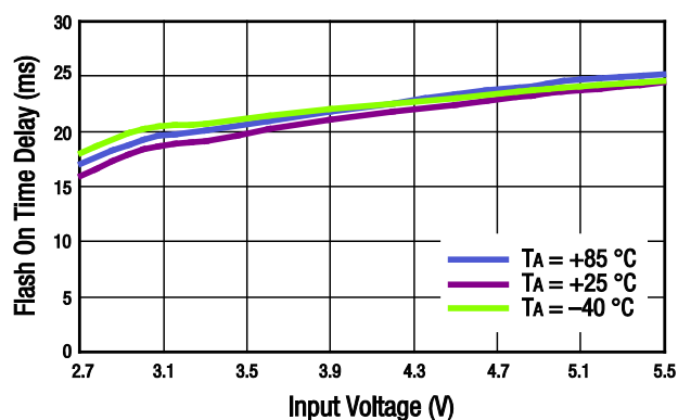
Figure 8. Flash On Time Delay vs Input Voltage
