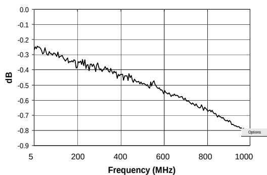
Amplitude Unbalance
