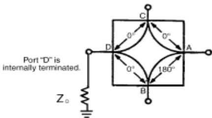
Figure 1. 2-way, In-Phase (180°) Power Divider/Summer, or ISO-T
