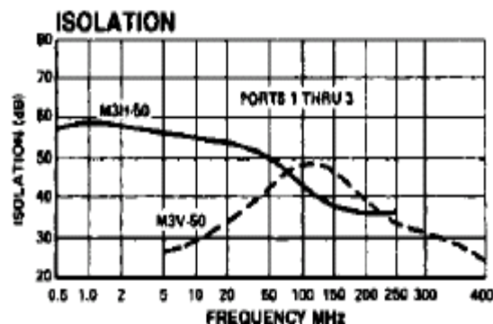
Isolation - Ports 1 - 3
