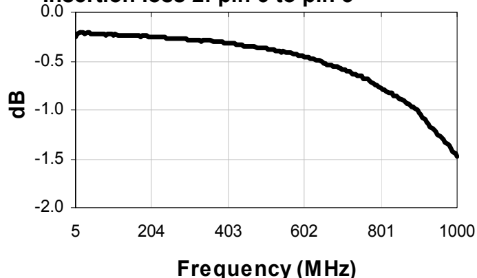
Insertion loss 2: pin 6 to pin 3
