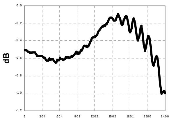
Amplitude Unbalance
