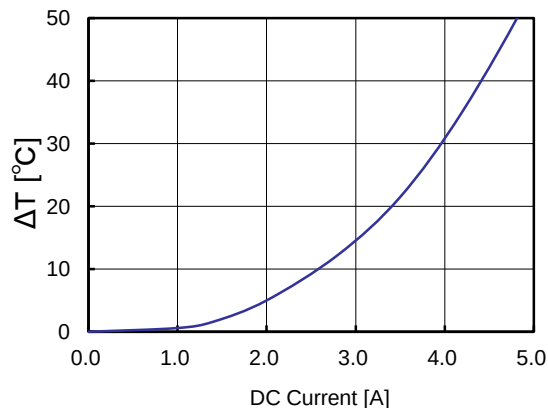
Temperature Rise vs DC Current
