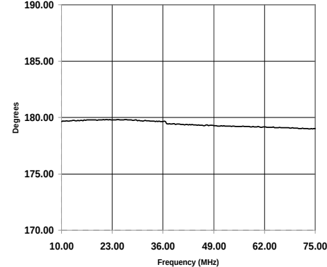
Phase Unbalance
