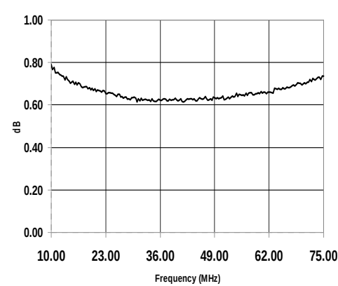
Amplitude Unbalance
