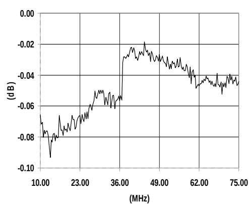
Amplitude Unbalance
