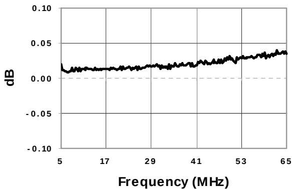
Amplitude Unbalance
