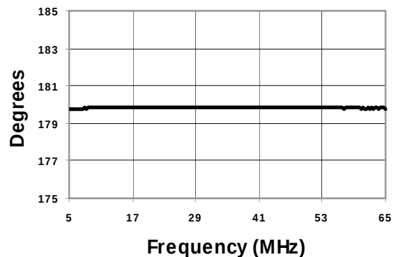
Phase Balance
