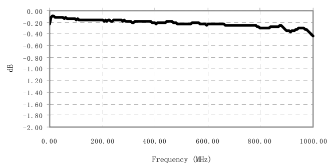
Insertion Loss
