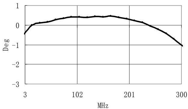
Phase Balance
