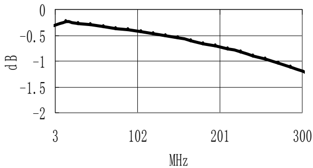
Amplitude Balance
