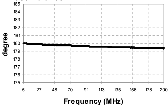
Phase Balance
