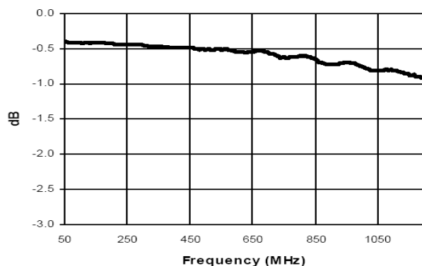
Insertion Loss Pin 4-3
