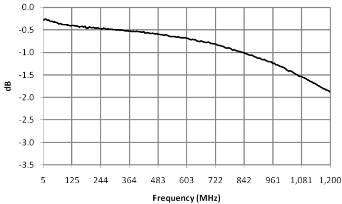
MABA-011029 insertion_loss_1_p1_2
