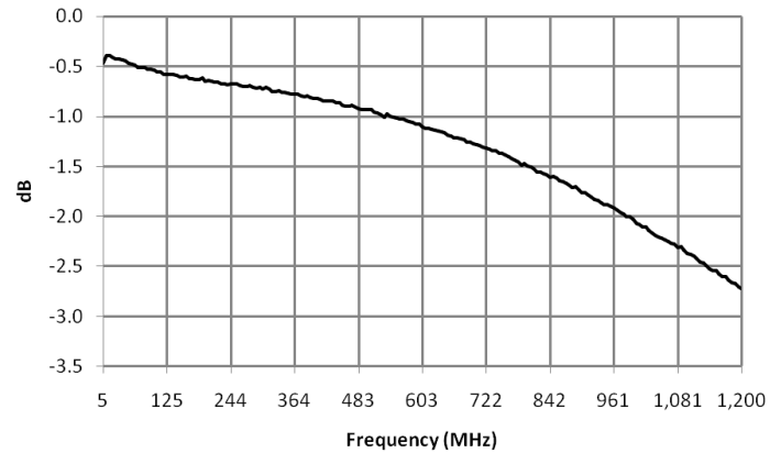
MABA-011029 insertion_loss_2_p1_3
