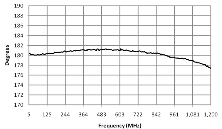
MABA-011029 phase_balance
