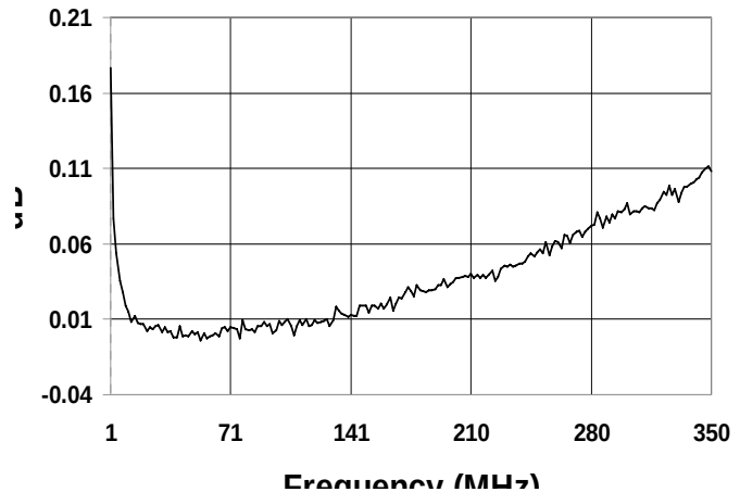
Amplitude Unbalance
