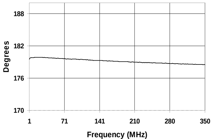
Phase Balance
