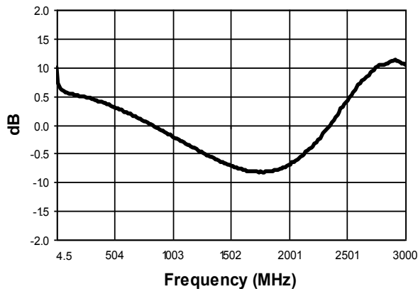
Amplitude Balance
