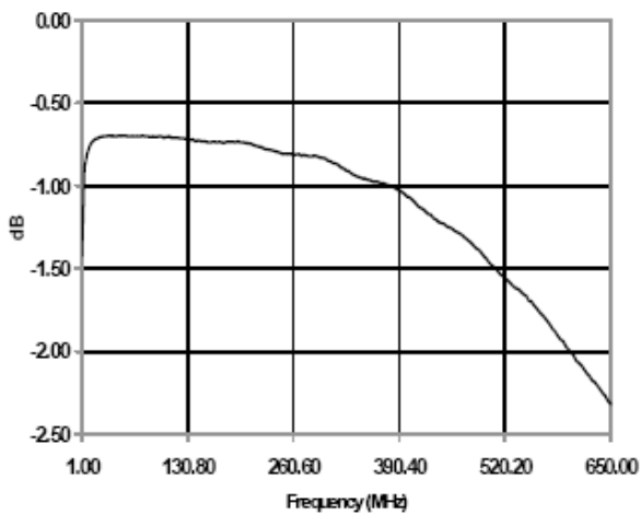
Amplitude Unbalance
