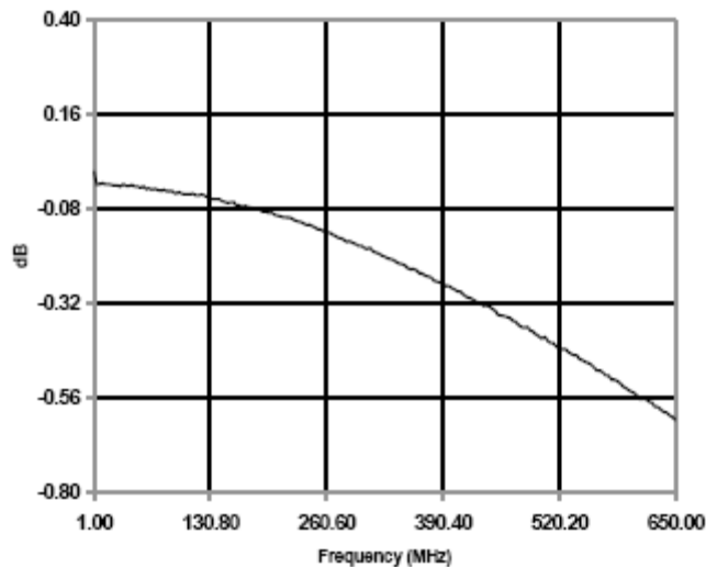
Amplitude Unbalance
