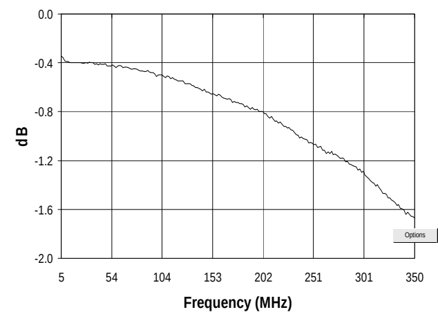
Primary to Secondary Dot Insertion Loss
