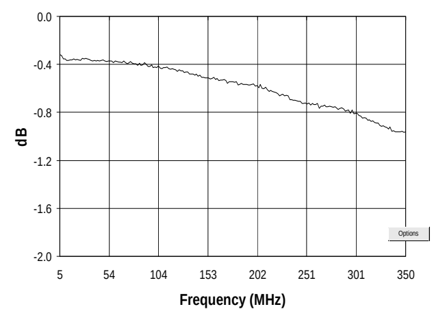
Primary to Secondary Insertion Loss
