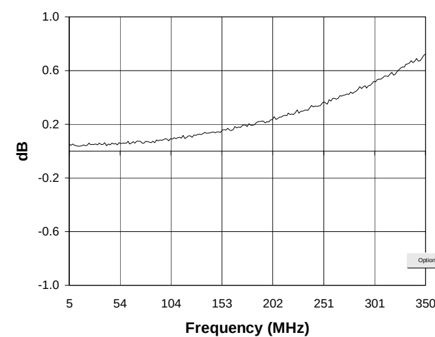
Amplitude Imbalance
