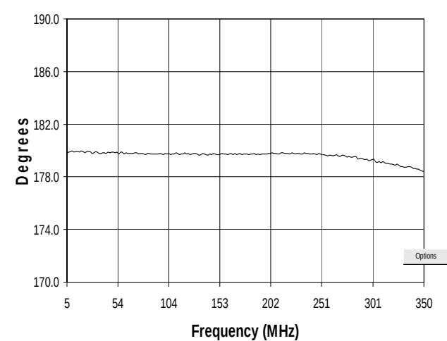
Phase Imbalance
