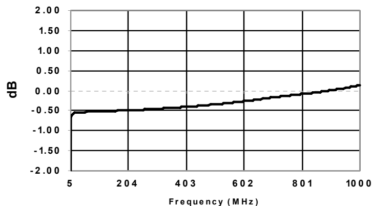
Amplitude Balance
