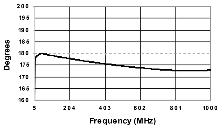
Phase Balance
