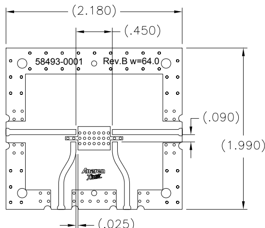
Test Board
