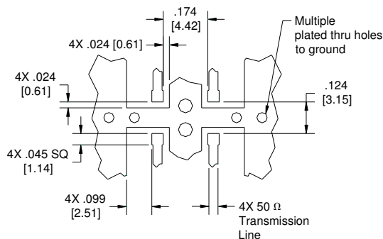
Dimensions are in Inches [Millimeters] 1P603S Mounting Footprint
