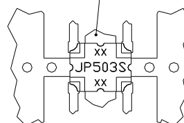
Part Is Symmetric About All Axis
