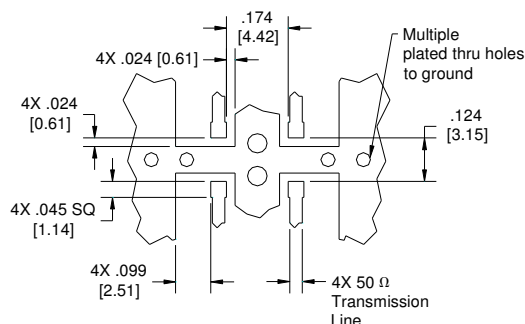
Dimensions are in Inches [Millimeters] JP503S Mounting Footprint
